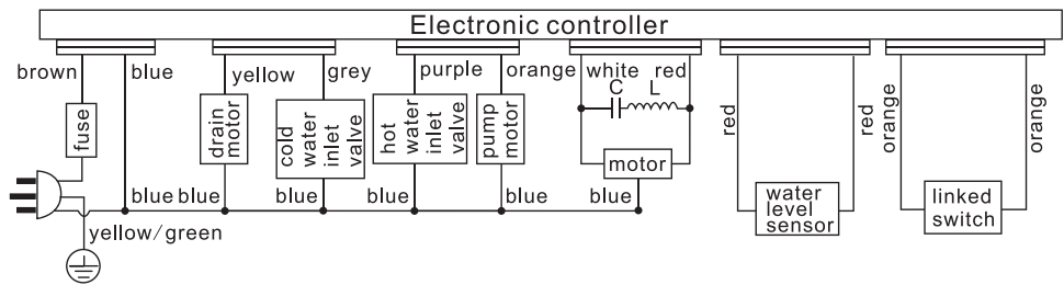
Circuit Diagram
