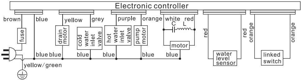
Circuit Diagram
